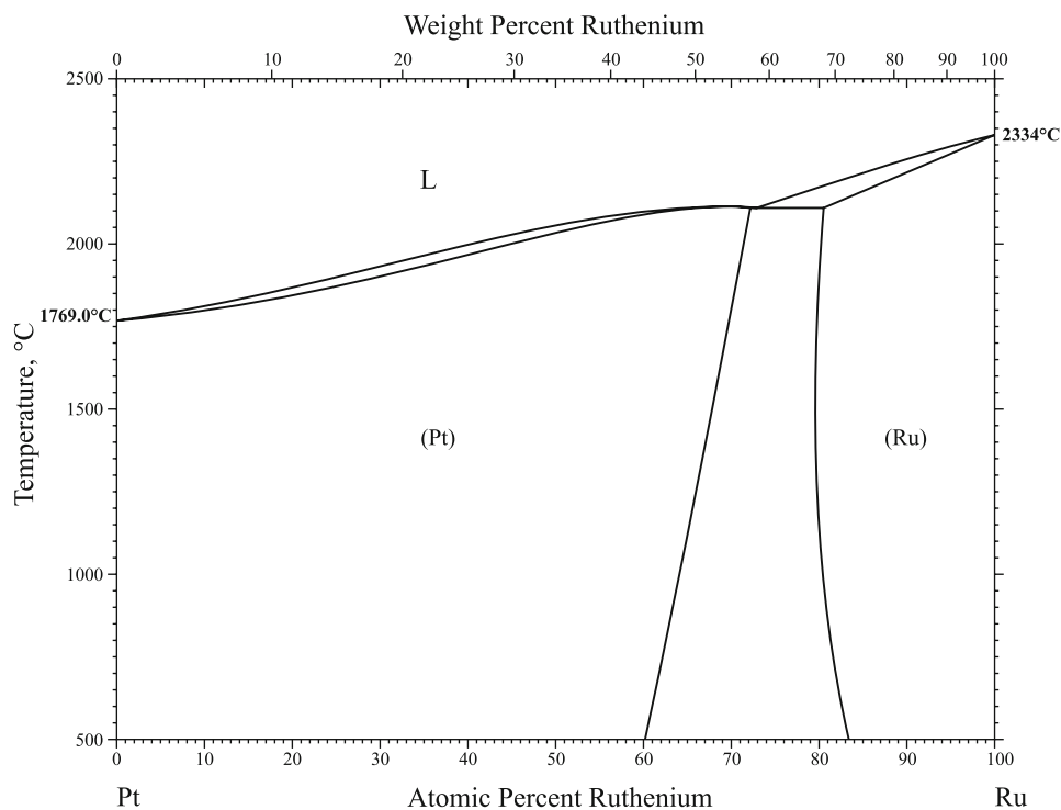
Fig. 1 Pt-Ru phase diagram
